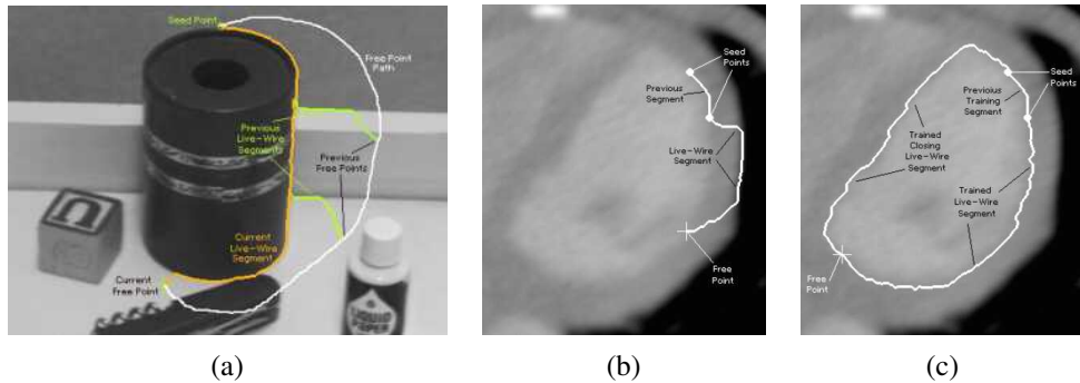
Figure 7.48 Intelligent scissors: (a) as the mouse traces the white path, the scissors follow the orange path along the object boundary (the green curves show intermediate positions) (Mortensen and Barrett 1995) © 1995 ACM; (b) regular scissors can sometimes jump to a stronger (incorrect) boundary; (c) after training to the previous segment, similar edge profiles are preferred (Mortensen and Barrett 1998) © 1995 Elsevier.
