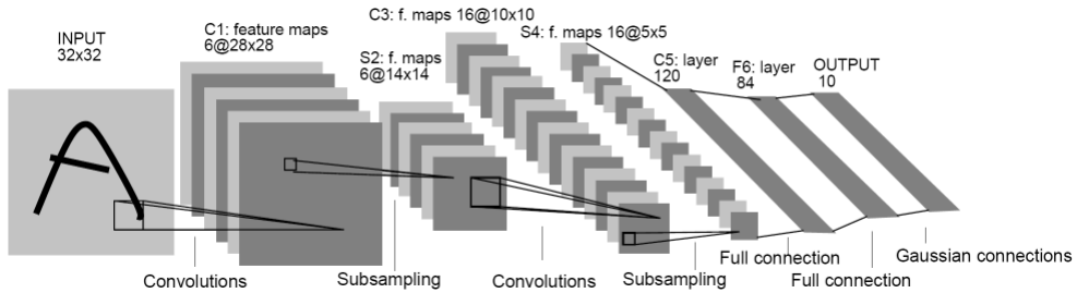
Figure 5.33 Architecture of LeNet-5 , a convolutional neural network for digit recognition ( LeCun, Bottou et al. 1998 ) © 1998 IEEE. This network uses multiple channels in each layer and alternates multi-channel convolutions with downsampling operations, followed by some fully connected layers that produce one activation for each of the 10 digits being classified.
