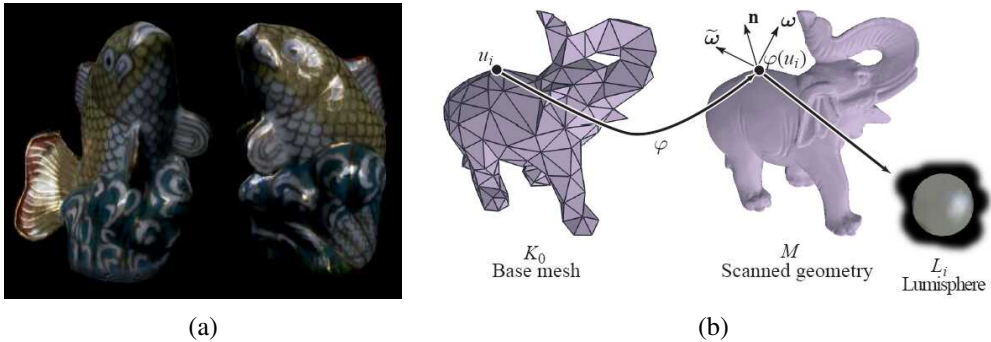
Figure 14.11 Surface light fields (Wood, Azuma et al. 2000) © 2000 ACM: (a) example of a highly specular object with strong inter-reflections; (b) the surface light field stores the light emanating from each surface point in all visible directions as a “Lumisphere”.
