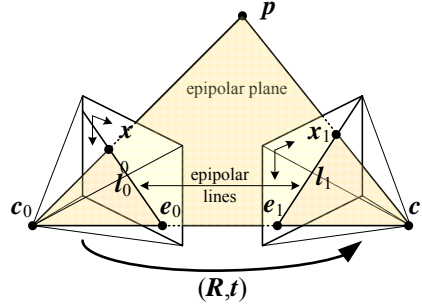
Figure 11.12 Epipolar geometry: The vectors \mathbf{t} = \mathbf{c}_1 - \mathbf{c}_0 , \mathbf{p} - \mathbf{c}_0 and \mathbf{p} - \mathbf{c}_1 are co-planar and define the basic epipolar constraint expressed in terms of the pixel measurements \mathbf{x}_0 and \mathbf{x}_1 .
