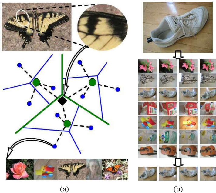
Figure 7.30 Scalable recognition using a vocabulary tree (Nistér and Stewénus 2006) © 2006 IEEE. (a) Each MSER elliptical region is converted into a SIFT descriptor, which is then quantized by comparing it hierarchically to some prototype descriptors in a vocabulary tree. Each leaf node stores its own inverted index (sparse list of non-zero tf-idf counts) into images that contain that feature. (b) A recognition result, showing a query image (top row) being indexed into a database of 6000 test images and correctly finding the corresponding four images.
