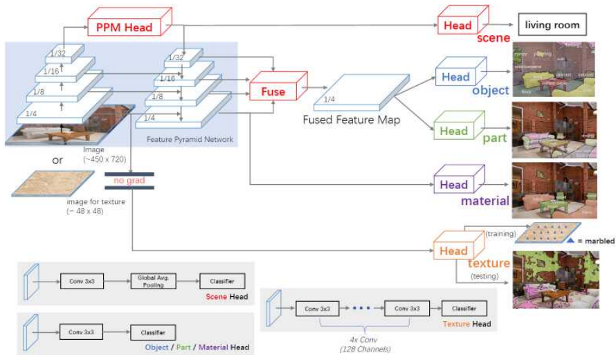
Figure 6.34 The UPerNet framework for Unified Perceptual Parsing. (Xiao, Liu et al. 2018) © 2018 Springer. A Feature Pyramid Network (FPN) backbone is appended with a Pyramid Pooling Module (PPM) before feeding it into the top-down branch of the FPN. Various layers of the FPN and/or PPM are fed into different heads, including a scene head for image classification, object and part heads from the fused FPN features, a material head operating on the finest level of the FPN, and a texture head that does not participate in the FPN fine tuning. The bottom gray squares give more details into some of the heads.
