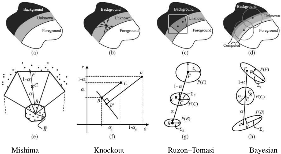
Figure 10.42 Image matting algorithms (Chuang, Curless et al. 2001) © 2001 IEEE. Mishima’s algorithm models global foreground and background color distribution as polyhedral surfaces centered around the mean background (blue) color. Knockout uses a local color estimate of foreground and background for each pixel and computes \alpha along each color axis. Ruzon and Tomasi’s algorithm locally models foreground and background colors and variances. Chuang et al.’s Bayesian matting approach computes a MAP estimate of (fractional) foreground color and opacity given the local foreground and background distributions.
