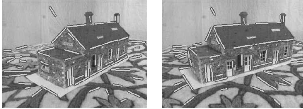
Figure 11.23 Two images of a toy house along with their matched 3D line segments (Schmid and Zisserman 1997) © 1997 Springer.
