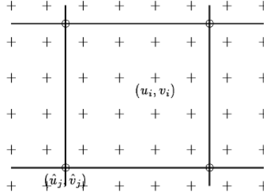
Figure 9.7 Spline motion field: the displacement vectors \mathbf{u}_i = (u_i, v_i) are shown as pluses (+) and are controlled by the smaller number of control vertices \hat{\mathbf{u}}_j = (\hat{u}_j, \hat{v}_j) , which are shown as circles (○).
