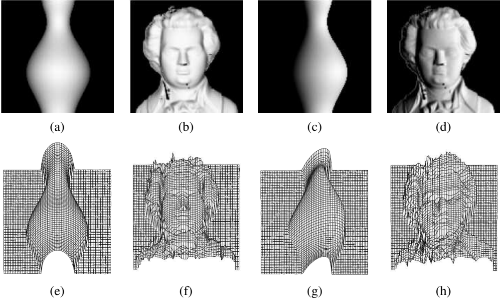
Figure 13.2 Synthetic shape from shading (Zhang, Tsai et al. 1999) © 1999 IEEE: shaded images, (a–b) with light from in front (0, 0, 1) and (c–d) with light the front right (1, 0, 1) ; (e–f) corresponding shape from shading reconstructions using the technique of Tsai and Shah (1994).
