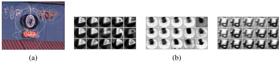
Figure 7.28 Visual words obtained from elliptical normalized affine regions (Sivic and Zisserman 2009) © 2009 IEEE. (a) Affine covariant regions are extracted from each frame and clustered into visual words using k -means clustering on SIFT descriptors with a learned Mahalanobis distance. (b) The central patch in each grid shows the query and the surrounding patches show the nearest neighbors.
