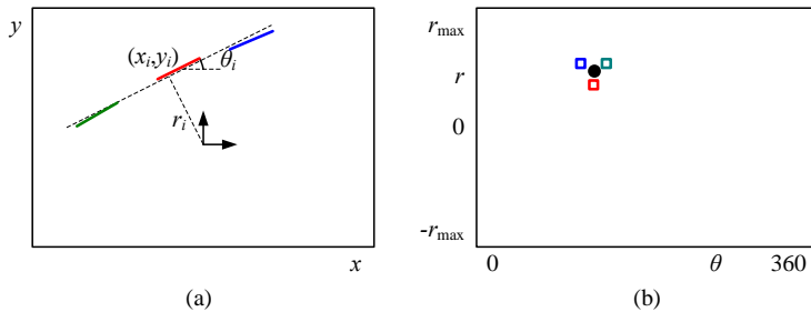
Figure 7.52 Oriented Hough transform: (a) an edgel re-parameterized in polar (r, \theta) coordinates, with \hat{\mathbf{n}}_i = (\cos \theta_i, \sin \theta_i) and r_i = \hat{\mathbf{n}}_i \cdot \mathbf{x}_i ; (b) (r, \theta) accumulator array, showing the votes for the three edgels marked in red, green, and blue.
