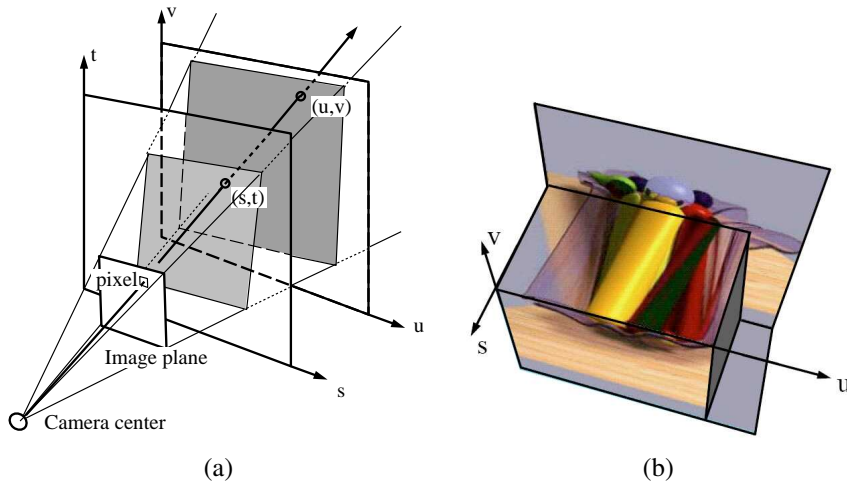
Figure 14.9 The Lumigraph (Gortler, Grzeszczuk et al. 1996) © 1996 ACM: (a) a ray is represented by its 4D two-plane parameters (s, t) and (u, v) ; (b) a slice through the 3D light field subset (u, v, s) .
