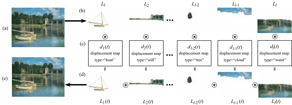
Figure 14.16 Animating still pictures (Chuang, Goldman et al. 2005) © 2005 ACM. (a) The input still image is manually segmented into (b) several layers. (c) Each layer is then animated with a different stochastic motion texture (d) The animated layers are then composited to produce (e) the final animation
