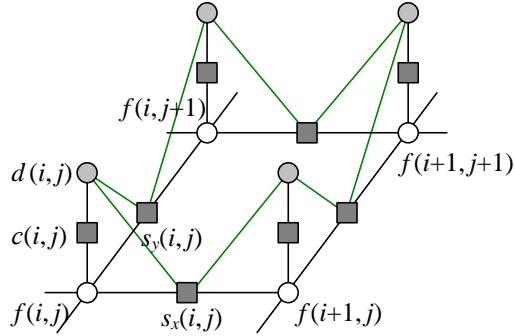
Figure 4.19 Graphical model for a conditional random field (CRF). The additional green edges show how combinations of sensed data influence the smoothness in the underlying MRF prior model, i.e., s_x(i, j) and s_y(i, j) in (4.42) depend on adjacent d(i, j) values. These additional links (factors) enable the smoothness to depend on the input data. However, they make sampling from this MRF more complex.
