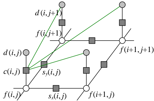
Figure 4.20 Graphical model for a discriminative random field (DRF). The additional green edges show how combinations of sensed data, e.g., d(i, j + 1) , influence the data term for f(i, j) . The generative model is therefore more complex, i.e., we cannot just apply a simple function to the unknown variables and add noise.
