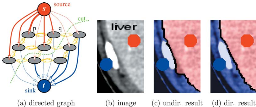
Figure 4.24 Segmentation with a directed graph cut (Boykov and Funka-Lea 2006) © 2006 Springer: (a) directed graph; (b) image with seed points; (c) the undirected graph incorrectly continues the boundary along the bright object; (d) the directed graph correctly segments the light gray region from its darker surround.
