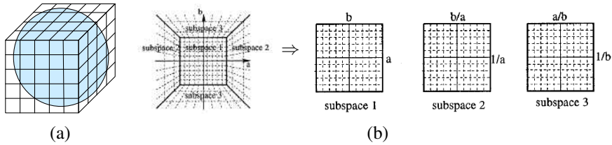
Figure 7.54 Cube map representation for line equations and vanishing points: (a) a cube map surrounding the unit sphere; (b) projecting the half-cube onto three subspaces (Tuytelaars, Van Gool, and Proesmans 1997) © 1997 IEEE.
