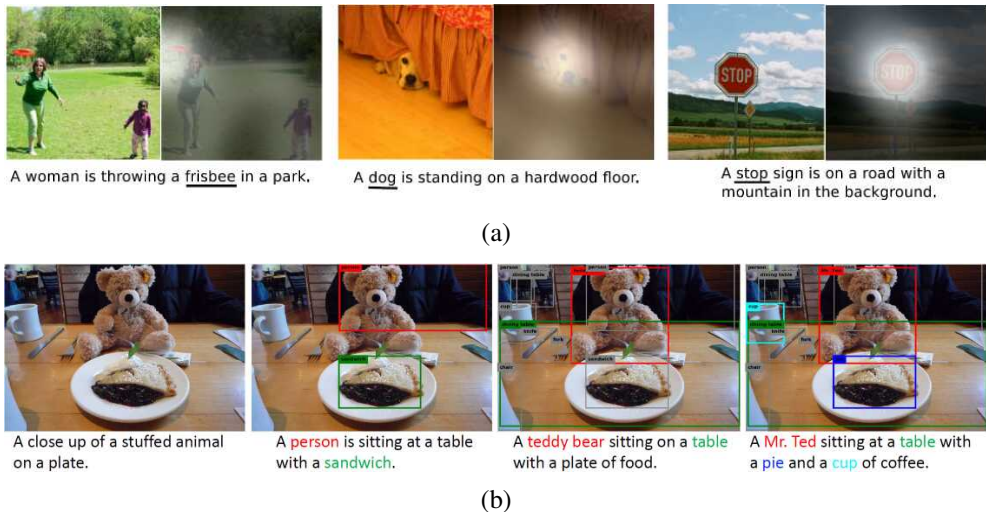
Figure 6.45 Image captioning with attention: (a) The “Show, Attend, and Tell” system, which uses hard attention to align generated words with image regions © Xu, Ba et al. (2015); (b) Neural Baby Talk captions generated using different detectors, showing the association between words and grounding regions (Lu, Yang et al. 2018) © 2018 IEEE.
