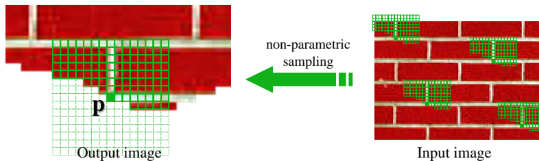
Figure 10.51 Texture synthesis using non-parametric sampling (Efros and Leung 1999). The value of the newest pixel p is randomly chosen from similar local (partial) patches in the source texture (input image). (Figure courtesy of Alyosha Efros.)
