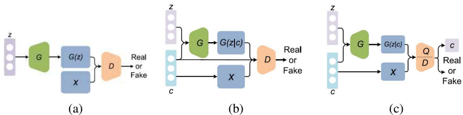
Figure 5.56 Generative adversarial network (GAN) architectures from (Pan, Yu et al. 2019) © 2019 IEEE. (a) In a regular GAN, random “latent” noise vectors z are fed into a generator network G , which produces synthetic “fake” images x' = G(z) . The job of the discriminator D is to tell the fake images apart from real samples x . (b) In a conditional GAN (cGAN), the network iterates (during training) over all the classes that we wish to synthesize. The generator G gets both a class id c and a random noise vector z as input, and the discriminator D gets the class id as well and needs to determine if its input is a real member of the given class. (c) The discriminator in an InfoGAN does not have access to the class id, but must instead infer it from the samples it is given.
