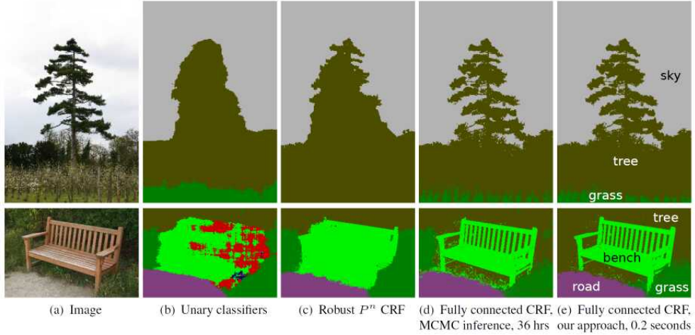
Figure 4.22 Pixel-level classification with a fully connected CRF, from © Krähenbühl and Koltun (2011). The labels in each column describe the image or algorithm being run, which include a robust P^n CRF (Kohli, Ladický, and Torr 2009) and a very slow MCMC optimization algorithm.
