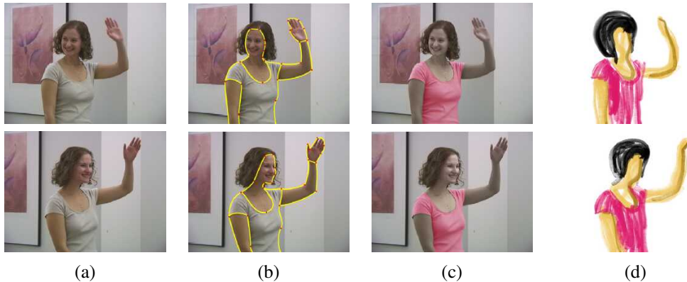
Figure 7.50 Keyframe-based rotoscoping (Agarwala, Hertzmann et al. 2004) © 2004 ACM: (a) original frames; (b) rotoscoped contours; (c) re-colored blouse; (d) rotoscoped hand-drawn animation.
