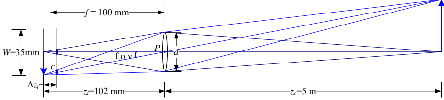
Figure 2.19 A thin lens of focal length f focuses the light from a plane a distance z_o in front of the lens at a distance z_i behind the lens, where \frac{1}{z_o} + \frac{1}{z_i} = \frac{1}{f} . If the focal plane (vertical gray line next to c ) is moved forward, the images are no longer in focus and the circle of confusion c (small thick line segments) depends on the distance of the image plane motion \Delta z_i relative to the lens aperture diameter d . The field of view (f.o.v.) depends on the ratio between the sensor width W and the focal length f (or, more precisely, the focusing distance z_i , which is usually quite close to f ).
