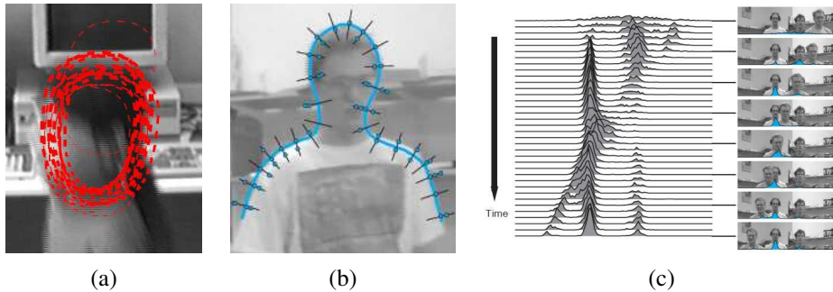
Figure 7.47 Head tracking using CONDENSATION (Isard and Blake 1998) © 1998 Springer: (a) sample set representation of head estimate distribution; (b) multiple measurements at each control vertex location; (c) multi-hypothesis tracking over time.
