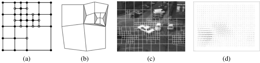
Figure 9.9 Quadtree spline-based motion estimation (Szeliski and Shum 1996) © 1996 IEEE: (a) quadtree spline representation, (b) which can lead to cracks, unless the white nodes are constrained to depend on their parents; (c) deformed quadtree spline mesh overlaid on grayscale image; (d) flow field visualized as a needle diagram.
