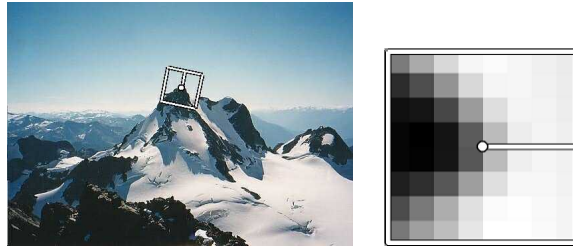
Figure 7.17 MOPS descriptors are formed using an 8 \times 8 sampling of bias and gain normalized intensity values, with a sample spacing of five pixels relative to the detection scale (Brown, Szeliski, and Winder 2005) © 2005 IEEE. This low frequency sampling gives the features some robustness to interest point location error and is achieved by sampling at a higher pyramid level than the detection scale.
