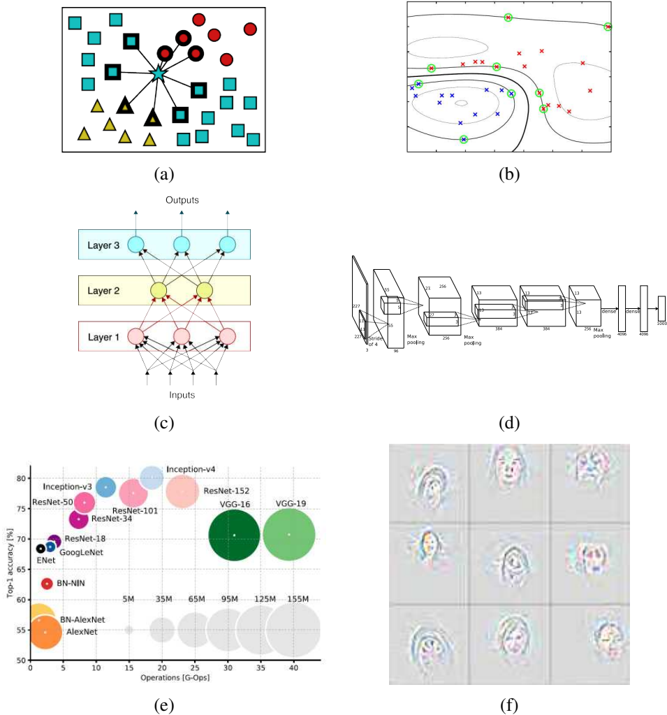
Figure 5.1 Machine learning and deep neural networks: (a) nearest neighbor classification © Glassner (2018) ; (b) Gaussian kernel support vector machine ( Bishop 2006 ) © 2006 Springer; (c) a simple three-layer network © Glassner (2018) ; (d) the SuperVision deep neural network, courtesy of Matt Dietke after ( Krizhevsky, Sutskever, and Hinton 2012 ); (e) network accuracy vs. size and operation counts ( Canziani, Culurciello, and Paszke 2017 ) © 2017 IEEE; visualizing network features ( Zeiler and Fergus 2014 ) © 2014 Springer.
