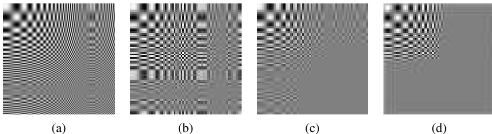
Figure 2.26 Aliasing of a two-dimensional signal: (a) original full-resolution image; (b) downsampled 4\times with a 25% fill factor box filter; (c) downsampled 4\times with a 100% fill factor box filter; (d) downsampled 4\times with a high-quality 9-tap filter. Notice how the higher frequencies are aliased into visible frequencies with the lower quality filters, while the 9-tap filter completely removes these higher frequencies.
