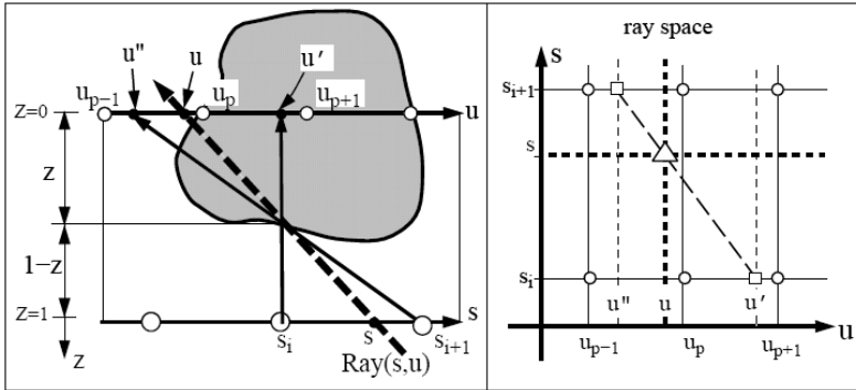
Figure 14.10 Depth compensation in the Lumigraph (Gortler, Grzeszczuk et al. 1996) © 1996 ACM. To resample the (s, u) dashed light ray, the u parameter corresponding to each discrete s_i camera location is modified according to the out-of-plane depth z to yield new coordinates u and u' ; in (u, s) ray space, the original sample ( \triangle ) is resampled from the (s_i, u') and (s_{i+1}, u'') samples, which are themselves linear blends of their adjacent ( \circ ) samples.
