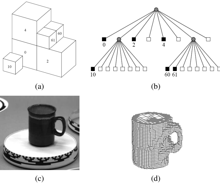
Figure 12.27 Volumetric octree reconstruction from binary silhouettes (Szeliski 1993) © 1993 Elsevier: (a) octree representation and its corresponding (b) tree structure; (c) input image of an object on a turntable; (d) computed 3D volumetric octree model.
