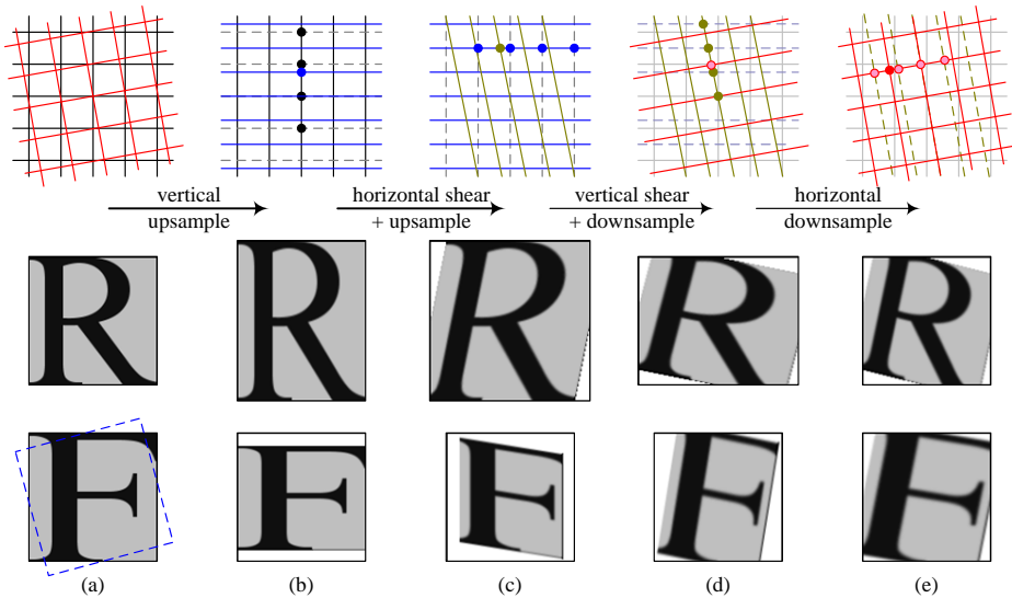
Figure 3.50 Four-pass rotation (Szeliski, Winder, and Uyttendaele 2010): (a) original pixel grid, image, and its Fourier transform; (b) vertical upsampling; (c) horizontal shear and upsampling; (d) vertical shear and downsampling; (e) horizontal downsampling. The general affine case looks similar except that the first two stages perform general resampling.
