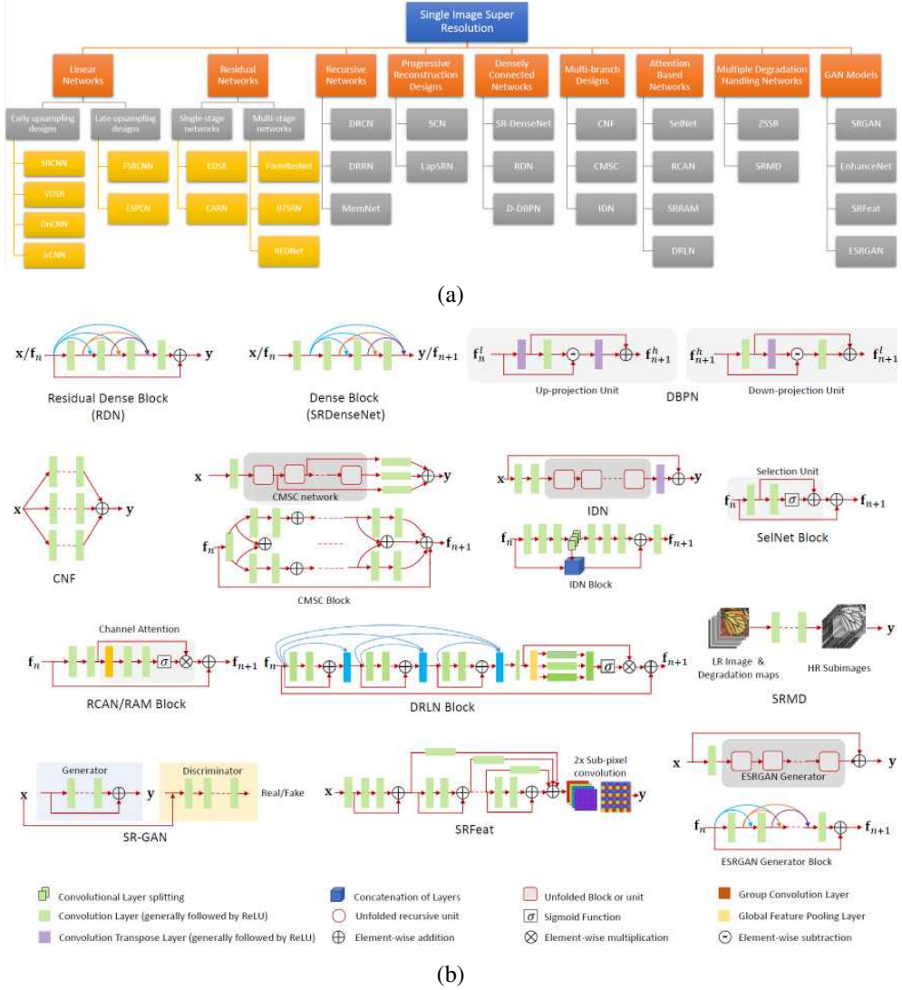
Figure 10.32 Recent deep neural network algorithms for single image super-resolution © 2019 (Anwar, Khan, and Barnes 2019): (a) a taxonomy of the algorithms based on their general approach; (b) schematic architectures for a subset of the algorithms.
