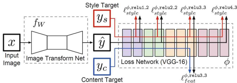
Figure 10.58 Network architecture for neural style transfer, which learns to transform images in one particular style (Johnson, Alahi, and Fei-Fei 2016) © 2016 Springer. During training, the content target image y_c is fed into the image transformation network as an input x , along with a style image y_s , and the network weights are updated so as to minimize the perceptual losses, i.e., the style reconstruction loss l_{style} and the feature reconstruction loss l_{feat} . The earlier network by Gatys, Ecker, and Bethge (2015) did not have an image transformation network, and instead used the losses to optimize the transformed image \hat{y} .
