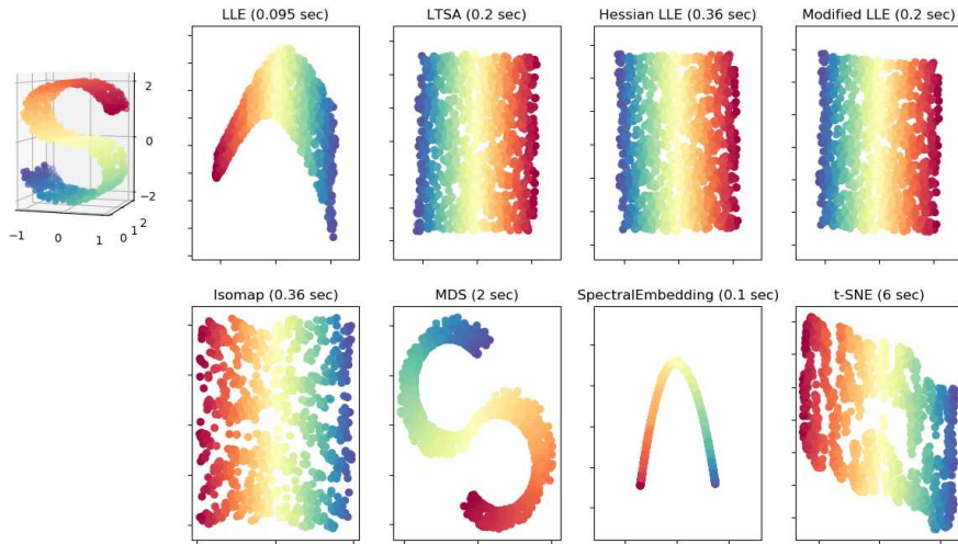
Figure 5.20 Examples of manifold learning, i.e., non-linear dimensionality reduction, applied to 1000 points with 10 neighbors each, from https://scikit-learn.org/stable/modules/manifold.html . The eight sample outputs were produced by eight different embedding algorithms, as described in the scikit-learn manifold learning documentation page.
