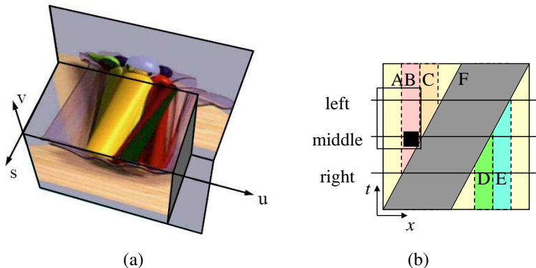
Figure 12.18 Epipolar plane image (EPI) (Gortler, Grzeszczuk et al. 1996) © 1996 ACM and a schematic EPI (Kang, Szeliski, and Chai 2001) © 2001 IEEE. (a) The Lumigraph (light field) (Section 14.3) is the 4D space of all light rays passing through a volume of space. Taking a 2D slice results in all of the light rays embedded in a plane and is equivalent to a scanline taken from a stacked EPI volume. Objects at different depths move sideways with velocities (slopes) proportional to their inverse depth. Occlusion (and translucency) effects can easily be seen in this representation. (b) The EPI corresponding to Figure 12.19 showing the three images (middle, left, and right) as slices through the EPI volume. The spatially and temporally shifted window around the black pixel is indicated by the rectangle, showing the right image is not being used in matching.
