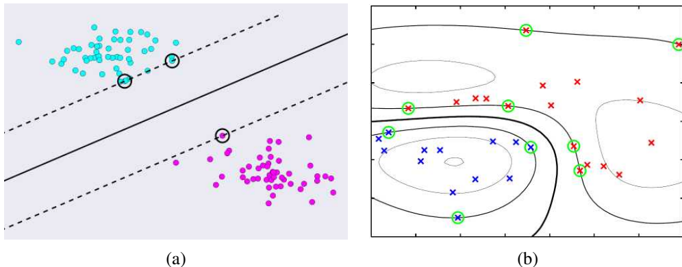
Figure 5.11 (a) A support vector machine (SVM) finds the linear decision surface (hyperplane) that maximizes the margin to the nearest training examples, which are called the support vectors © Glassner (2018). (b) A two-dimensional two class example of a Gaussian kernel support vector machine (Bishop 2006) © 2006 Springer. The red and blue \times s indicate the training samples, and the samples circled in green are the support vectors. The black lines indicate iso-contours of the kernel regression function, with the contours containing the blue and red support vectors indicating the \pm 1 contours and the dark contour in between being the decision surface.
