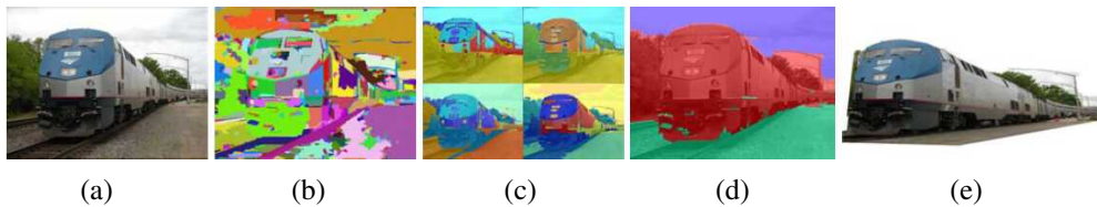
Figure 6.40 Automatic photo pop-up (Hoiem, Efros, and Hebert 2005a) © 2005 ACM: (a) input image; (b) superpixels are grouped into (c) multiple regions; (d) labelings indicating ground (green), vertical (red), and sky (blue); (e) novel view of resulting piecewise-planar 3D model.
