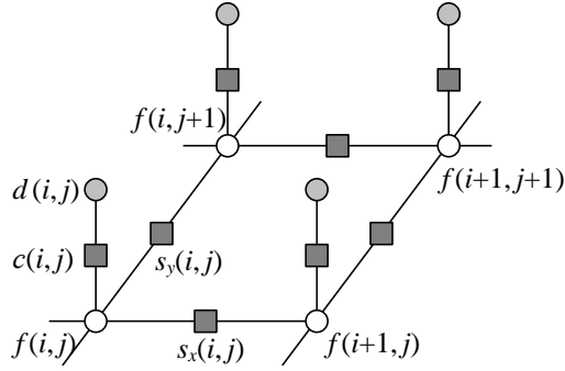
Figure 4.10 Graphical model interpretation of first-order regularization. The white circles are the unknowns f(i, j) while the dark circles are the input data d(i, j) . In the resistive grid interpretation, the d and f values encode input and output voltages and the black squares denote resistors whose conductance is set to s_x(i, j) , s_y(i, j) , and c(i, j) . In the spring-mass system analogy, the circles denote elevations and the black squares denote springs. The same graphical model can be used to depict a first-order Markov random field (Figure 4.13).
