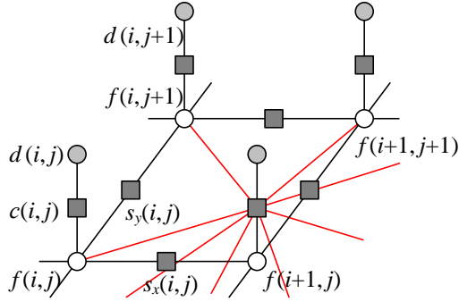
Figure 4.16 Graphical model for a Markov random field with a more complex measurement model. The additional colored edges show how combinations of unknown values (say, in a sharp image) produce the measured values (a noisy blurred image). The resulting graphical model is still a classic MRF and is just as easy to sample from, but some inference algorithms (e.g., those based on graph cuts) may not be applicable because of the increased network complexity, since state changes during the inference become more entangled and the posterior MRF has much larger cliques.
