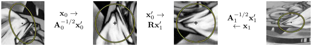
Figure 7.14 Affine normalization using the second moment matrices, as described by Mikolajczyk, Tuytelaars et al. (2005) © 2005 Springer. After image coordinates are transformed using the matrices \mathbf{A}_0^{-1/2} and \mathbf{A}_1^{-1/2} , they are related by a pure rotation \mathbf{R} , which can be estimated using a dominant orientation technique.
