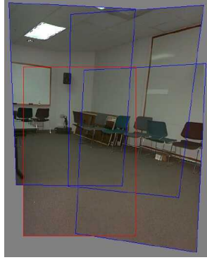
Figure 11.5 Four images taken with a hand-held camera registered using a 3D rotation motion model, which can be used to estimate the focal length of the camera (Szeliski and Shum 1997) © 2000 ACM.
