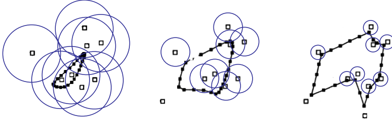
Figure 7.45 Elastic net: The open squares indicate the cities and the closed squares linked by straight line segments are the tour points. The blue circles indicate the approximate extent of the attraction force of each city, which is reduced over time. Under the Bayesian interpretation of the elastic net, the blue circles correspond to one standard deviation of the circular Gaussian that generates each city from some unknown tour point.
