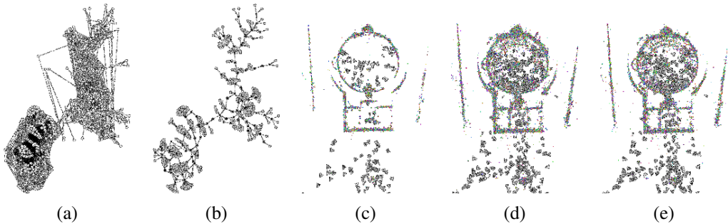
Figure 11.20 Large scale structure from motion using skeletal sets (Snavely, Seitz, and Szeliski 2008b) © 2008 IEEE: (a) original match graph for 784 images; (b) skeletal set containing 101 images; (c) top-down view of scene (Pantheon) reconstructed from the skeletal set; (d) reconstruction after adding in the remaining images using pose estimation; (e) final bundle adjusted reconstruction, which is almost identical.
