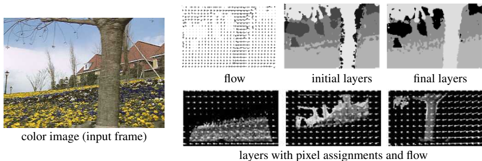
Figure 9.15 Layered motion estimation results (Wang and Adelson 1994) © 1994 IEEE.
