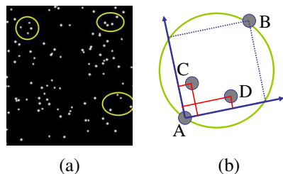
Figure 11.10 Locating star fields using astrometry, http://astrometry.net/ . (a) Input star field and some selected star quads. (b) The 2D coordinates of stars C and D are encoded relative to the unit square defined by A and B.
