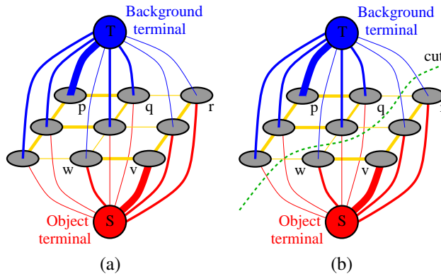
Figure B.5 Graph cuts for minimizing binary sub-modular MRF energies (Boykov and Jolly 2001) © 2001 IEEE: (a) energy function encoded as a max flow problem; (b) the minimum cut determines the region boundary.
