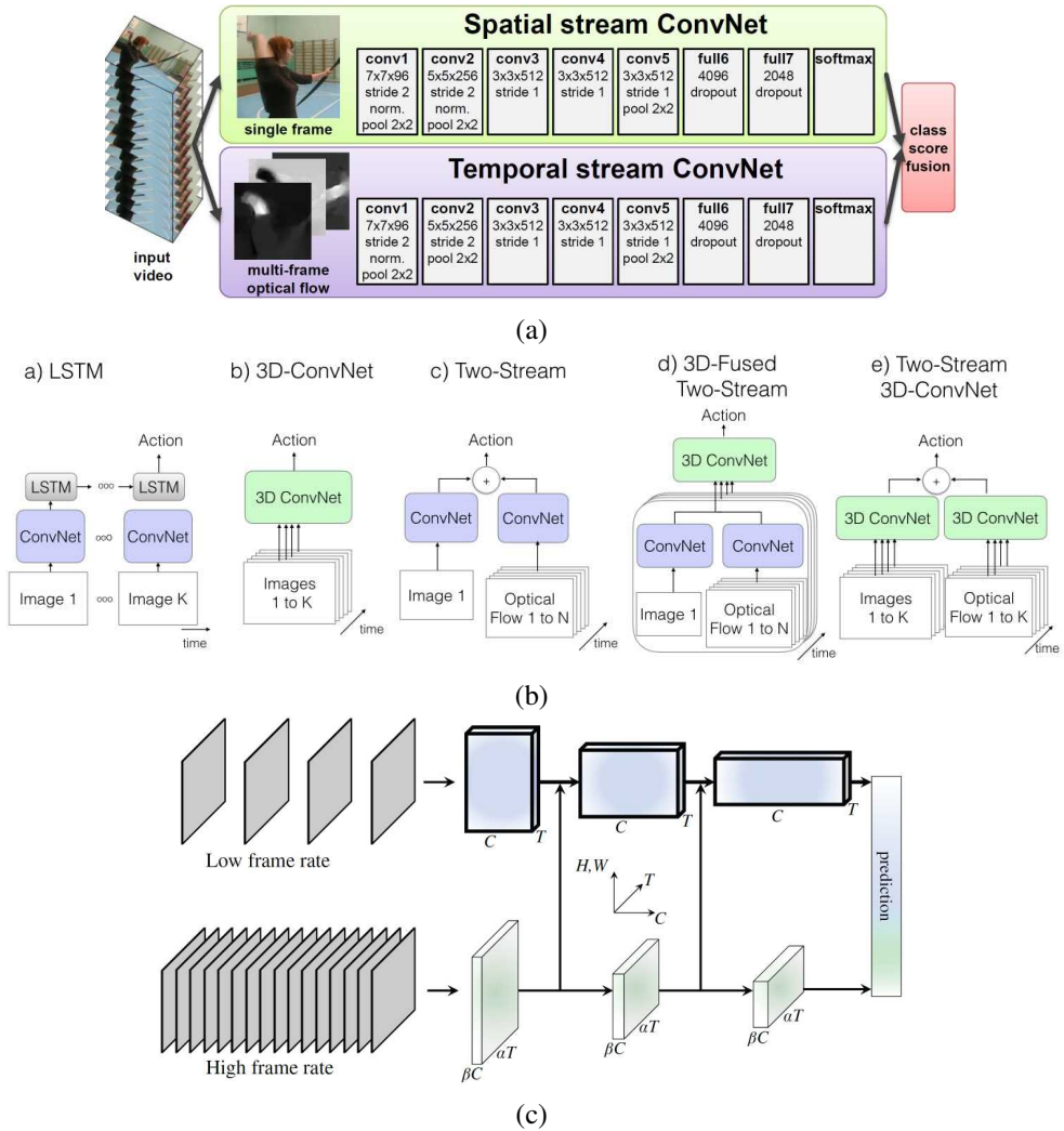
Figure 6.43 Video understanding using neural networks: (a) two-stream architecture for video classification © Simonyan and Zisserman (2014a); (b) some alternative video processing architectures (Carreira and Zisserman 2017) © 2017 IEEE; (c) a SlowFast network with a low frame rate, low temporal resolution Slow pathway and a high frame rate, higher temporal resolution Fast pathway (Feichtenhofer, Fan et al. 2019) © 2019 IEEE.
