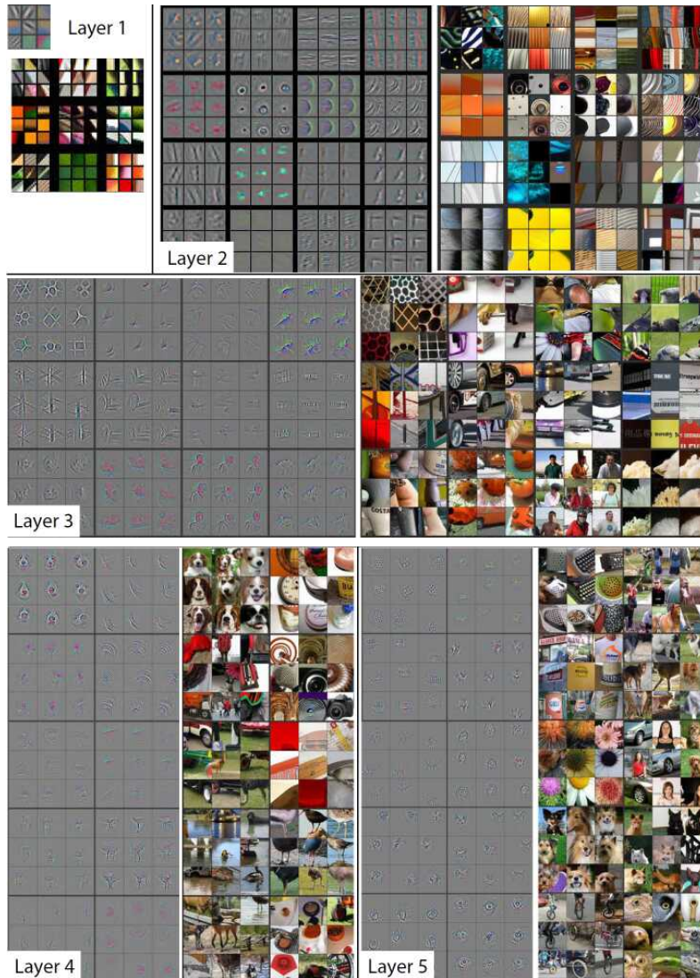
Figure 5.47 Visualizing network weights and features, from (Zeiler and Fergus 2014) © 2014 Springer. Each visualized convolutional layer is taken from a network adapted from the SuperVision net of Krizhevsky, Sutskever, and Hinton (2012). The 3 \times 3 subimages denote the top 9 responses in one feature map (channel in a given layer) projected back into pixel space (higher layers project to larger pixel patches), with the color images on the right showing the most responsive image patches from the validation set, and the grayish signed images on the left showing the corresponding maximum stimulus pre-images.
