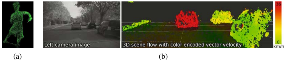
Figure 12.21 Three-dimensional scene flow: (a) computed from a multi-camera dome surrounding the dancer shown in Figure 12.2h–j (Vedula, Baker et al. 2005) © 2005 IEEE; (b) computed from stereo cameras mounted on a moving vehicle (Wedel, Rabe et al. 2008) © 2008 Springer.
