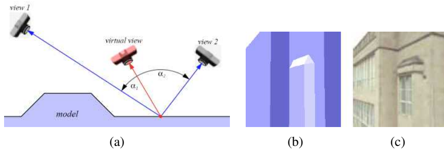
Figure 14.3 View-dependent texture mapping (Debevec, Taylor, and Malik 1996) © 1996 ACM. (a) The weighting given to each input view depends on the relative angles between the novel (virtual) view and the original views; (b) simplified 3D model geometry; (c) with view-dependent texture mapping, the geometry appears to have more detail (recessed windows).
