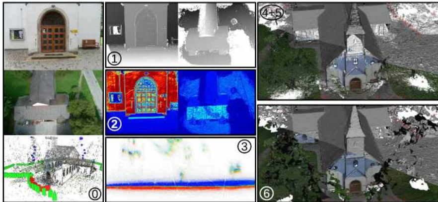
Figure 12.26 3D reconstruction pipeline from (Kuhn, Hirschmüller et al. 2017) © 2017 Springer: (0) structure from motion, (1) stereo matching using semi-global matching, (2) depth quality estimation, (3) probabilistic space occupancy, (4+5) probabilistic point optimization and outlier filtering, (6) triangulation. The images in (4+5) and (6) are half texture-mapped and half flat shaded to show more surface detail.
