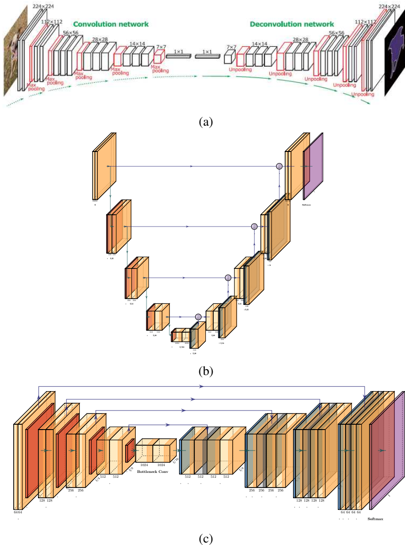
Figure 5.37 (a) The deconvolution network of Noh, Hong, and Han (2015) © 2015 IEEE and (b–c) the U-Net of Ronneberger, Fischer, and Brox (2015b), redrawn using the PlotNeuralNet LaTeX package by Matt Dietke. In addition to the fine-to-coarse-to-fine bottleneck used in (a), the U-Net also has skip connections between encoding and decoding layers at the same resolution.
