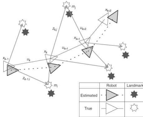
Figure 11.24 In simultaneous localization and mapping (SLAM), the system simultaneously estimates the positions of a robot and its nearby landmarks (Durrant-Whyte and Bailey 2006) © 2006 IEEE.
