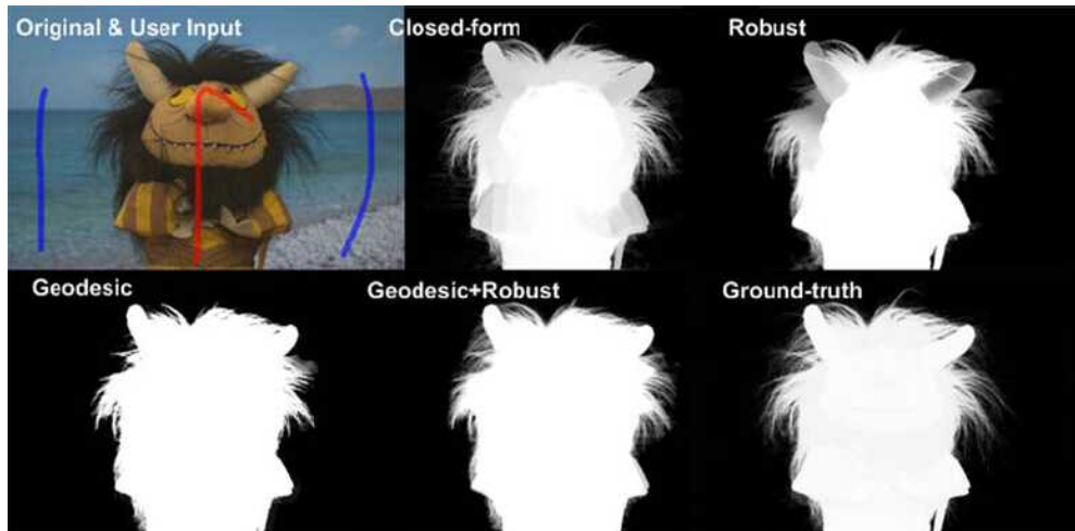
Figure 10.46 Comparative matting results with scribble-based inputs. Wang and Cohen (2009) describe the individual techniques being compared.
