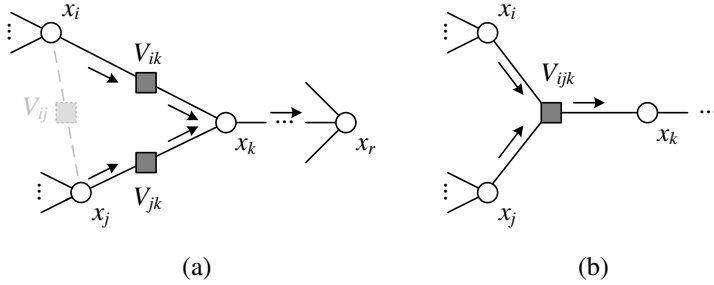
Figure B.4 Dynamic programming over a tree drawn as a factor graph. (a) To compute the lowest energy solution \hat{E}_k(x_k) at node x_k conditioned on the best solutions to the left of this node, we enumerate all possible values of \hat{E}_i(x_i) + V_{ik}(x_i, x_k) and pick the smallest one (and similarly for j ). (b) For higher-order cliques, we need to try all combinations of (x_i, x_j) in order to select the best possible configuration. The arrows show the basic flow of the computation. The lightly shaded factor V_{ij} in (a) shows an additional connection that turns the tree into a cyclic graph, for which exact inference cannot be efficiently computed.
