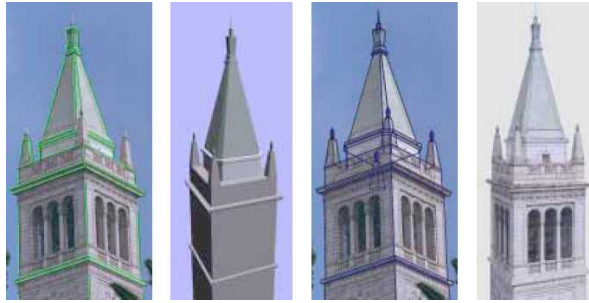
Figure 13.19 Interactive architectural modeling using the Façade system (Debevec, Taylor, and Malik 1996) © 1996 ACM: (a) input image with user-drawn edges shown in green; (b) shaded 3D solid model; (c) geometric primitives overlaid onto the input image; (d) final view-dependent, texture-mapped 3D model.
