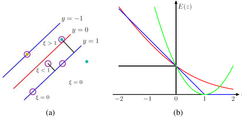
Figure 5.12 Support vector machine for overlapping class distributions (Bishop 2006) © 2006 Springer. (a) The green circled point is on the wrong side of the y = 1 decision contour and has a penalty of \xi = 1 - y > 0 . (b) The “hinge” loss used in support vector machines is shown in blue, along with a rescaled version of the logistic regression loss function, shown in red, the misclassification error in black, and the squared error in green.
