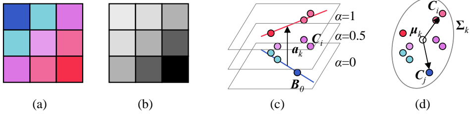
Figure 10.44 Color line matting (Levin, Lischinski, and Weiss 2008): (a) local 3 \times 3 patch of colors; (b) potential assignment of \alpha values; (c) foreground and background color lines, the vector \mathbf{a}_k joining their closest points of intersection, and the family of parallel planes of constant \alpha values, \alpha_i = \mathbf{a}_k \cdot (\mathbf{C}_i - \mathbf{B}_0) ; (d) a scatter plot of sample colors and the deviations from the mean \mu_k for two sample colors \mathbf{C}_i and \mathbf{C}_j .
