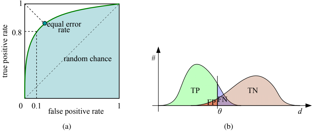
Figure 7.25 ROC curve and its related rates: (a) The ROC curve plots the true positive rate against the false positive rate for a particular combination of feature extraction and matching algorithms. Ideally, the true positive rate should be close to 1, while the false positive rate is close to 0. The area under the ROC curve (AUC) is often used as a single (scalar) measure of algorithm performance. Alternatively, the equal error rate is sometimes used. (b) The distribution of positives (matches) and negatives (non-matches) as a function of inter-feature distance d . As the threshold \theta is increased, the number of true positives (TP) and false positives (FP) increases.
