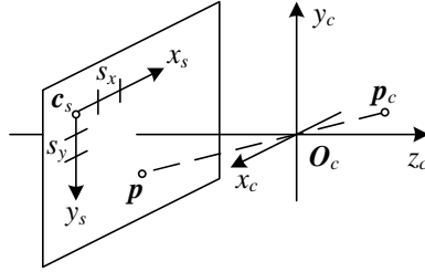
Figure 2.8 Projection of a 3D camera-centered point \mathbf{p}_c onto the sensor planes at location \mathbf{p} . \mathbf{O}_c is the camera center (nodal point), \mathbf{c}_s is the 3D origin of the sensor plane coordinate system, and s_x and s_y are the pixel spacings.
