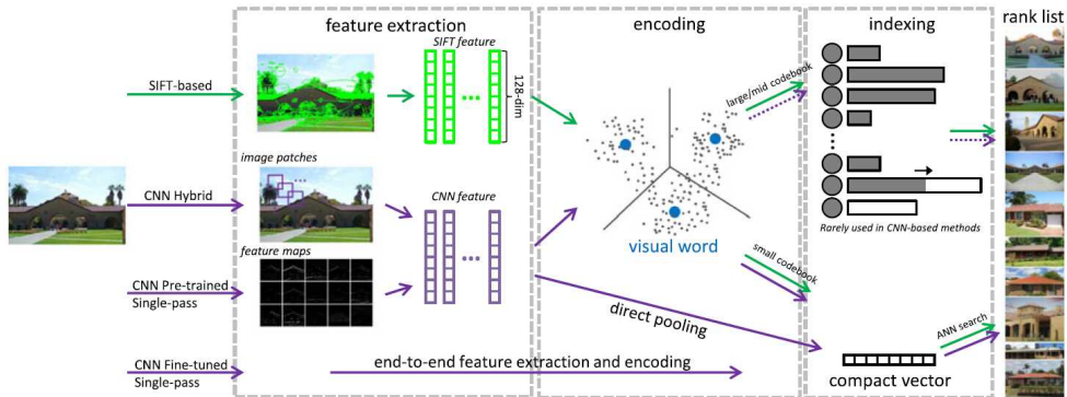
Figure 7.33 Typical pipeline for feature-based instance retrieval (Zheng, Yang, and Tian 2018) © 2018 IEEE, showing the feature extraction, encoding, and indexing portions, which are often collapsed when using a deep learning framework.
