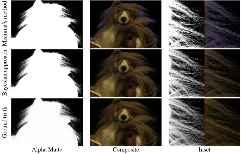
Figure 10.41 Blue-screen matting results (Chuang, Curless et al. 2001) © 2001 IEEE. Mishima's method produces visible blue spill (color fringing in the hair), while Chuang's Bayesian matting approach produces accurate results.
