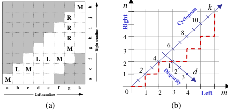
Figure 12.13 Stereo matching using dynamic programming, as illustrated by (a) Scharstein and Szeliski (2002) © 2002 Springer and (b) Kolmogorov, Criminisi et al. (2006) © 2006 IEEE . For each pair of corresponding scanlines, a minimizing path through the matrix of all pairwise matching costs (DSI) is selected. Lowercase letters (a–k) symbolize the intensities along each scanline. Uppercase letters represent the selected path through the matrix. Matches are indicated by M, while partially occluded points (which have a fixed cost) are indicated by L or R, corresponding to points only visible in the left or right images, respectively. Usually, only a limited disparity range is considered (0–4 in the figure, indicated by the non-shaded squares). The representation in (a) allows for diagonal moves while the representation in (b) does not. Note that these diagrams, which use the Cyclopean representation of depth, i.e., depth relative to a camera between the two input cameras, show an “unskewed” x - d slice through the DSI.
