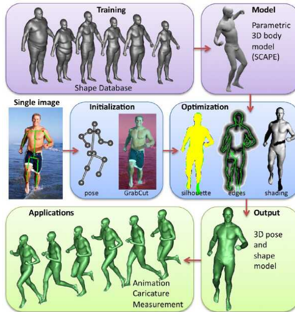
Figure 13.27 Estimating human shape and pose from a single image using a parametric 3D model (Guan, Weiss et al. 2009) © 2009 IEEE.
