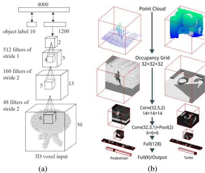
Figure 5.53 3D convolutional networks applied to volumetric data for objects detection: (a) 3D ShapeNets (Wu, Song et al. 2015) © 2015 IEEE; (b) VoxNet (Maturana and Scherer 2015) © 2015 IEEE.
