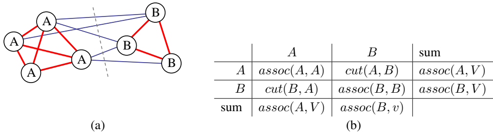
Figure 7.59 Sample weighted graph and its normalized cut: (a) a small sample graph and its smallest normalized cut; (b) tabular form of the associations and cuts for this graph. The assoc and cut entries are computed as area sums of the associated weight matrix \mathbf{W} . Normalizing the table entries by the row or column sums produces normalized associations and cuts N_{assoc} and N_{cut} .
