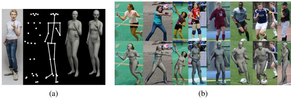
Figure 13.25 Whole body, expression, and gesture fitting from a single image using the SMPL-X model from (Pavlakos, Choutas et al. 2019) © 2019 IEEE: (a) estimating the major joints, skeleton, SMPL, and SMPL-X models from a single image; (b) qualitative results of SMPL-X for some in-the-wild images.
