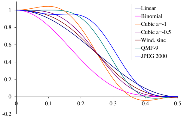
Figure 3.30 Frequency response for some 2\times decimation filters. The cubic a = -1 filter has the sharpest fall-off but also a bit of ringing; the wavelet analysis filters (QMF-9 and JPEG 2000), while useful for compression, have more aliasing.
