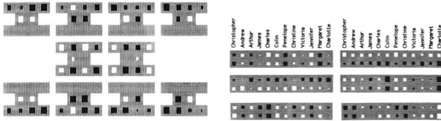
Figure 5.46 Hinton diagrams showing the weights connecting various layers in a neural network. From (Ackley, Hinton, and Sejnowski 1985) © 1985 Wiley.
