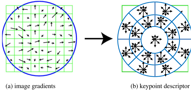
Figure 7.19 The gradient location-orientation histogram (GLOH) descriptor uses log-polar bins instead of square bins to compute orientation histograms (Mikolajczyk and Schmid 2005).
