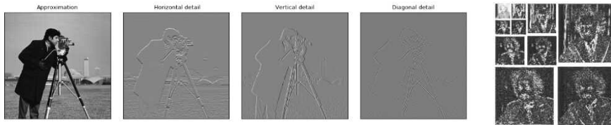
Figure 3.36 A wavelet decomposition of an image. The high-high components are in the lower right corner, while the base is in the upper left. Notice how the low-high and high-low components accentuate horizontal and vertical edges and gradients, while the high-high components store the less frequent mixed derivatives.
